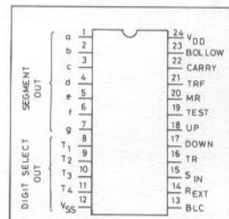
• TC5054P
